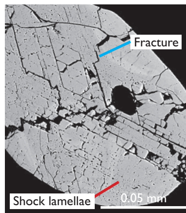
Interior polished surface: shock lamellae and fractures
