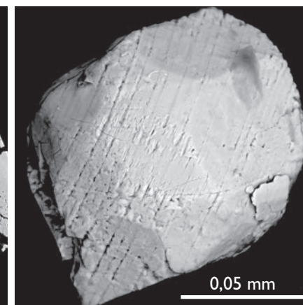
Crystal with partially annealed shock lamellae
