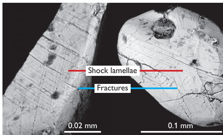
Zircon crystals with shock lamellae and fractures
